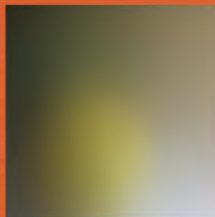
Acid Etch
